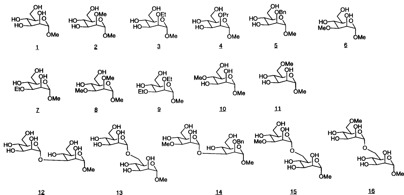
Figure 1. Ligands used in this study.
